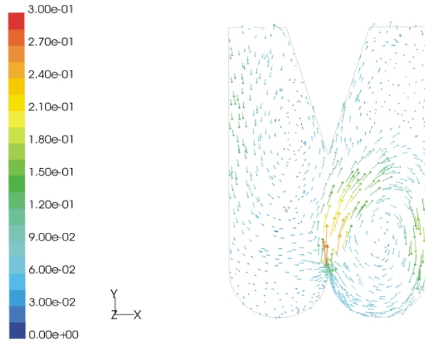
Velocity Vectors Colored By Velocity Magnitude (m/s) (Time=2.0314e+02) Oct 25, 2000 z=0.6m FLUENT 5.3 (3d, segregated, ke, unsteady)
